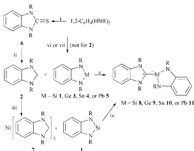
Scheme 1 Synthesis of carbene-group 14 metal(II) adducts 8–11 and compounds 2 , 3–7 (R = CH 2 Bu t ). Reagents: i, Cl 2 C=S, 2 NEt 3 ; ii, C 6 K; iii, \frac{1}{2} [Ni(cod) 2 ]; iv, 7 + 1 ; v, 2 + 1 , 3 , 4 or 5 ; vi, (M = Ge) 2 LiBu n , then [GeCl 2 (diox)]; vii, M[N(SiMe 3 ) 2 ] 2 (M = Sn or Pb).
